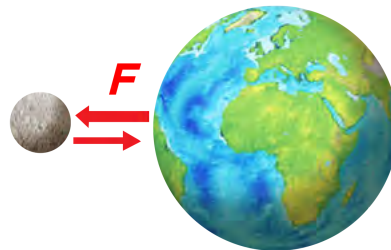
Stronger gravitational force
